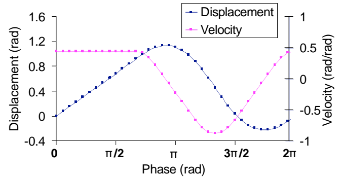
Figure 3: Displacement profile of an arbitrary cam profile.
