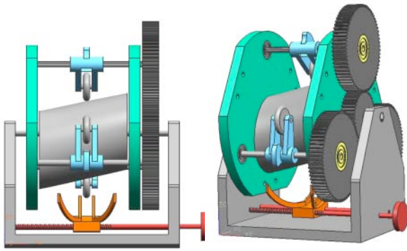
Figure 2: The front and isometric view of the transmission.
