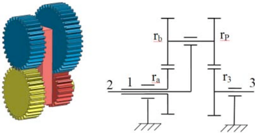
Figure 5: Planet gearset representative of the Cam-based IVT.
