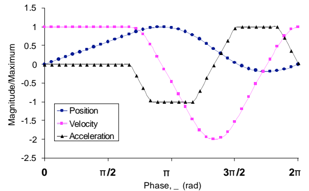
Figure 6: The follower's acceleration, velocity, and position as a function of cam rotation.
