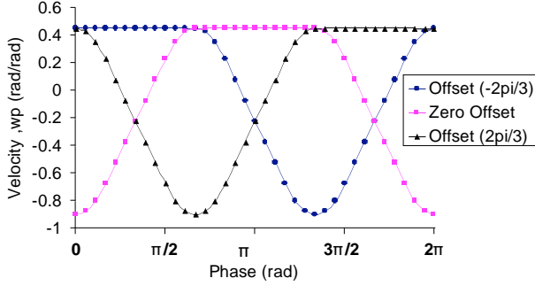
Figure 4: Overlay of the velocity profile in Figure 3 for three velocity profiles, showing the transfer of power between followers.
