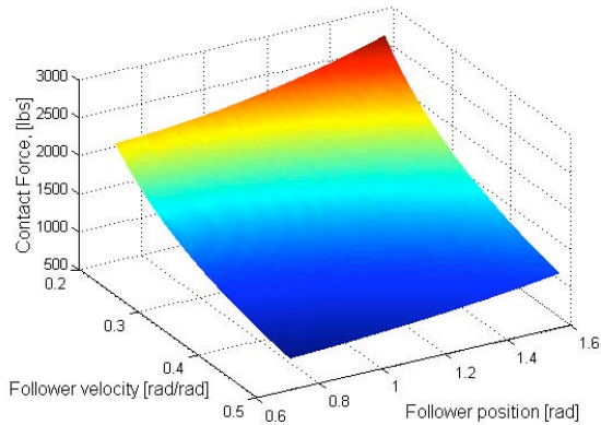
Figure 8: Contact force between roller and cam.
