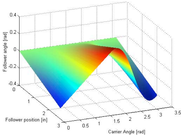
Figure 7: Follower position versus the carrier angle and the follower position along the length of the cam.
