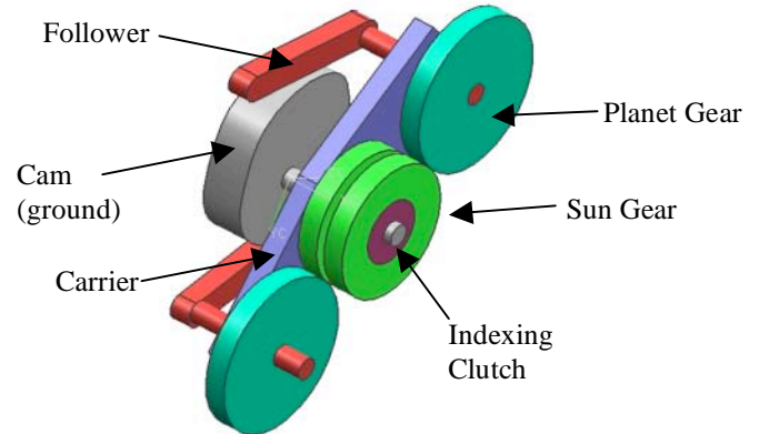
Figure 1: Simplified portrayal of the Cam-based IVT.
