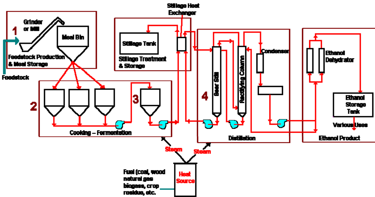
FIG. 1. Flowsheet for conversion of corn to fuel ethanol and animal food.
